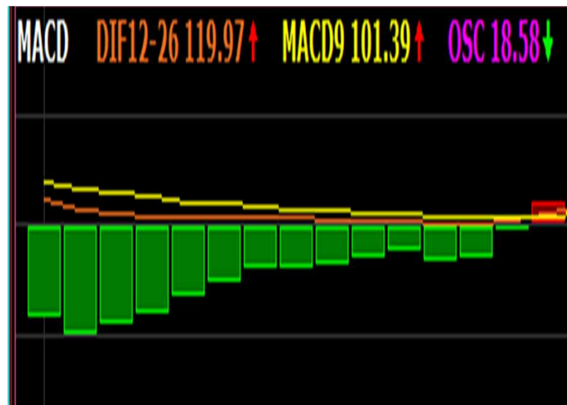
MACD
